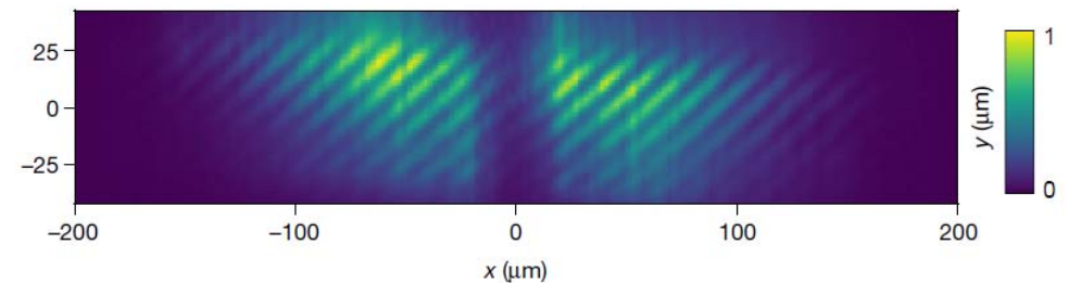
Interferogram of polariton condensate
