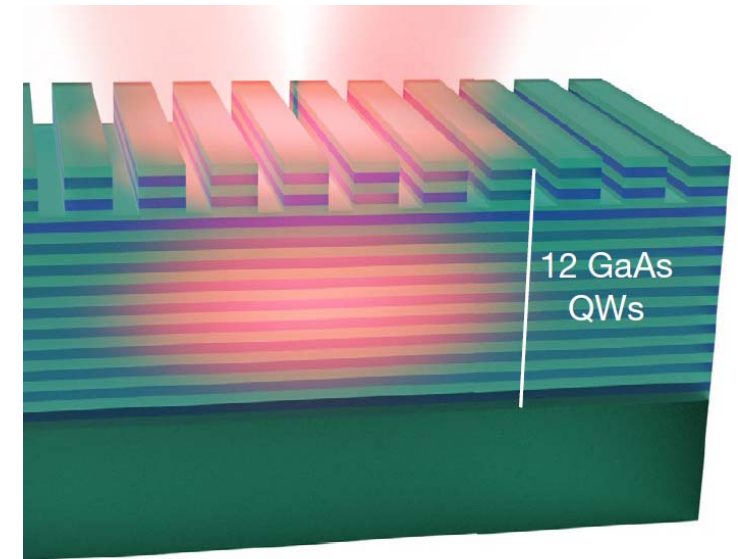
1D grating on GaAs QWs
