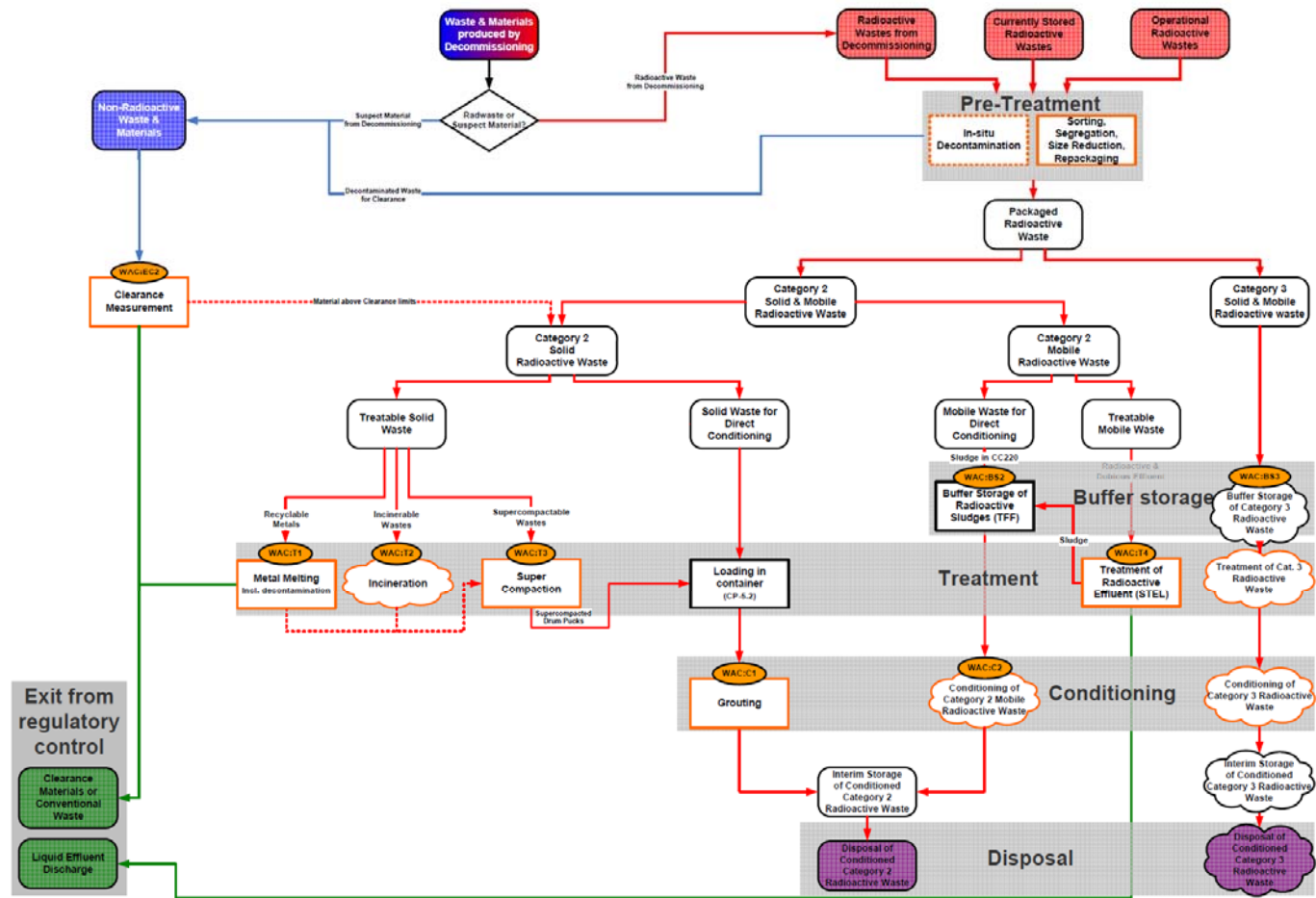
Waste streams @JRC Ispra
